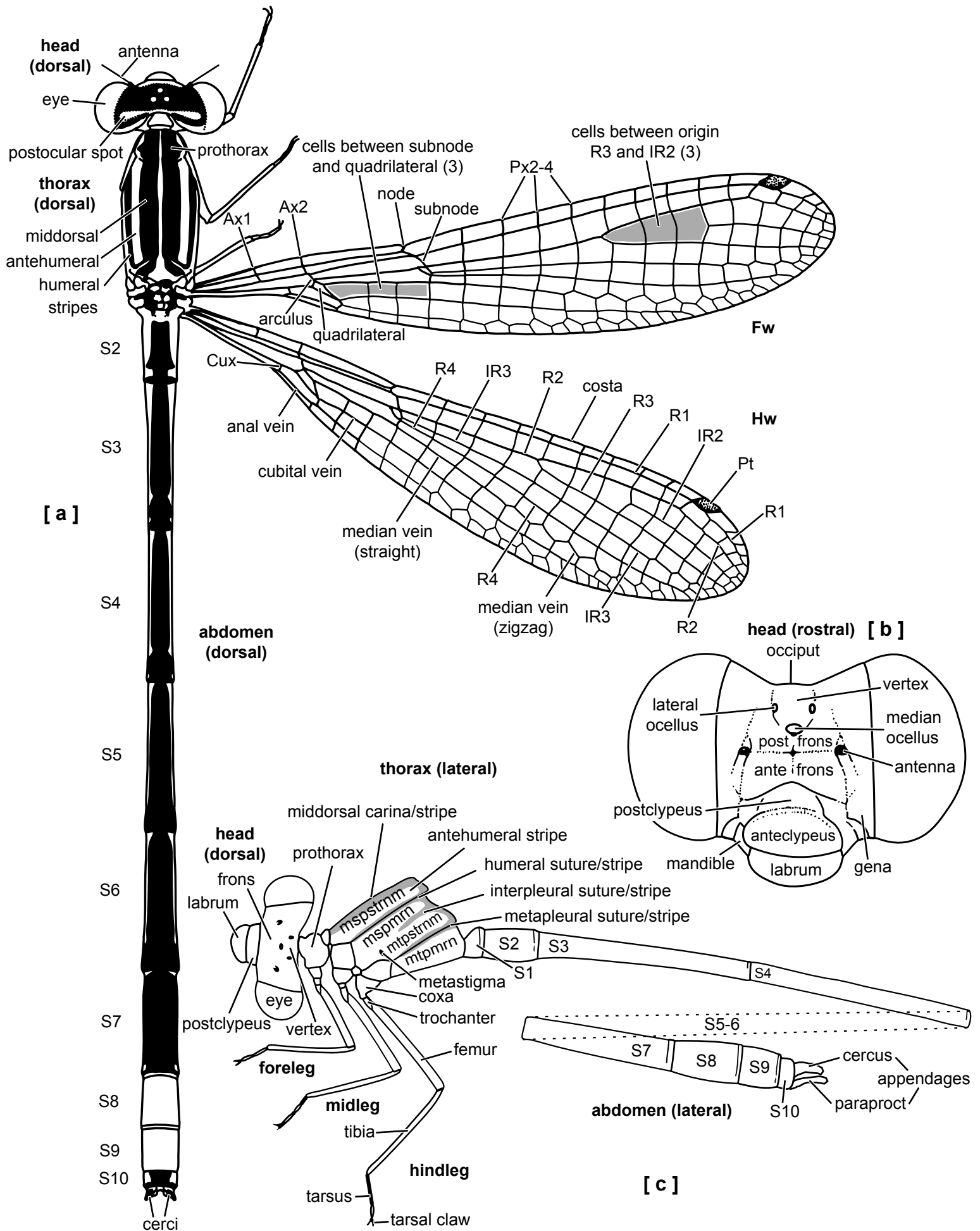
Fig. 2: Zygopteran morphology.
